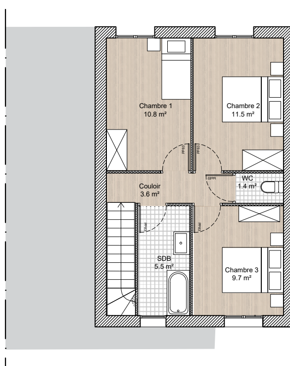
Plan R+1
